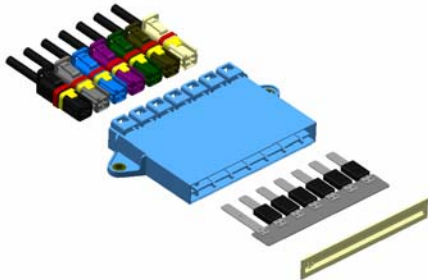
Sealed Pre-Fuse Box Solution
